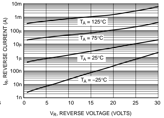
Figure 2. Reverse Characteristics
