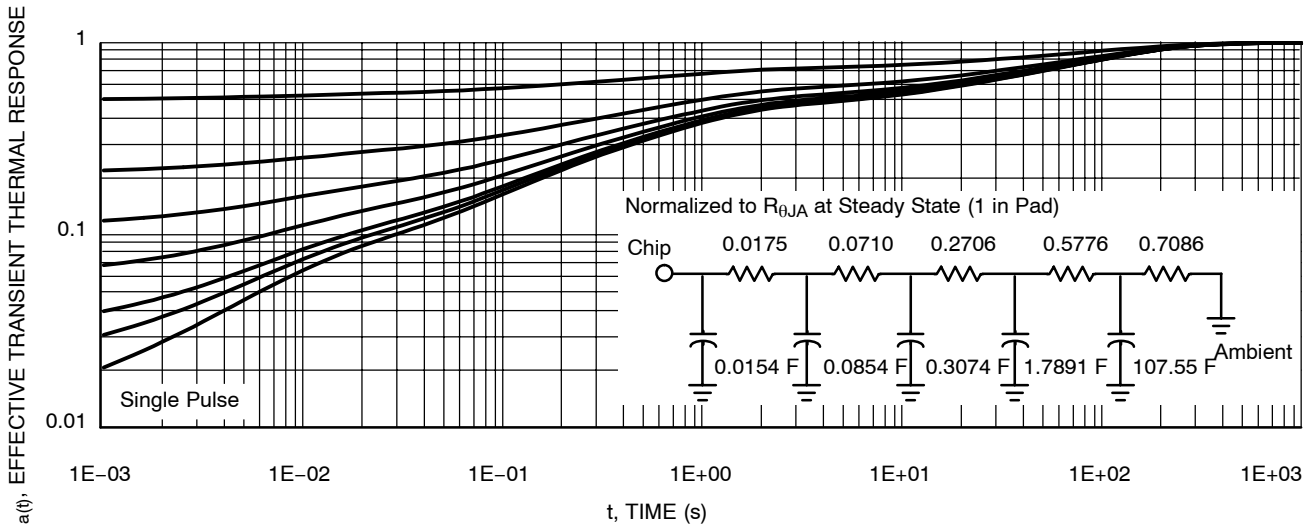
Figure 13. Thermal Response
