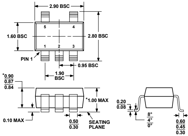
Figure 44. 5-Lead Thin Small Outline Transistor Package [TSOT] (UJ-5) Dimensions shown in millimeters
