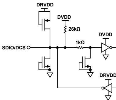
Figure 11. Equivalent SDIO/DCS or SMI SDFS Circuit
