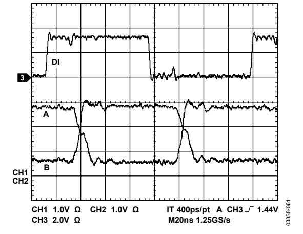
Figure 22. Driver Propagation Delay
