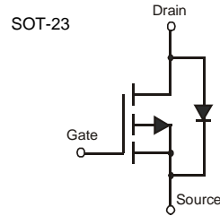
Internal Schematic
