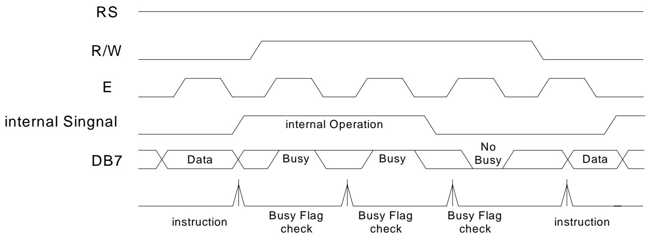
Example of 8-bit bus mode timing diagram
