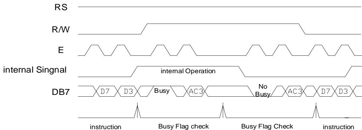
Example of 4-bit bus mode timing diagram
