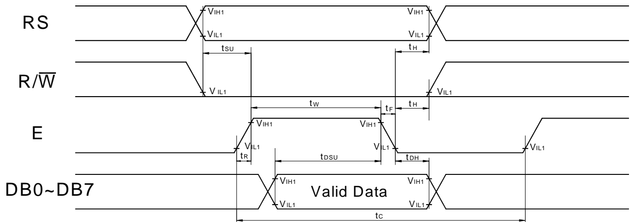
Fig. a Interface timing (data write)
