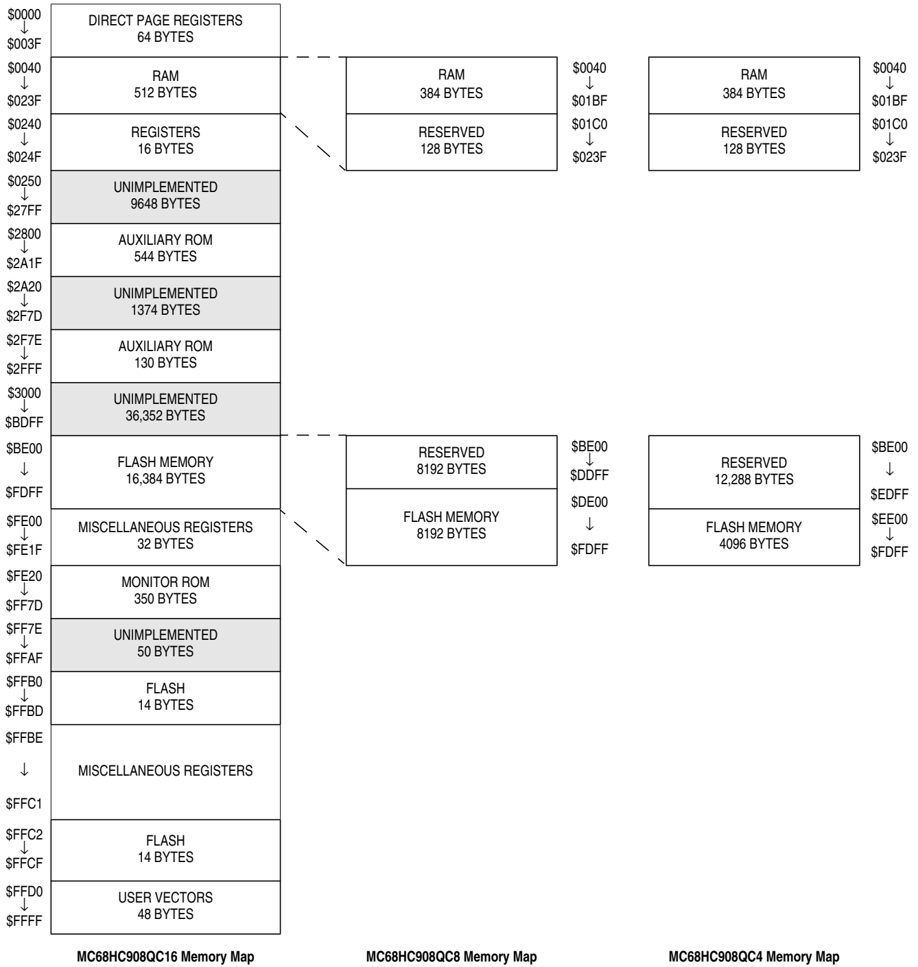
Figure 2-1. Memory Map
