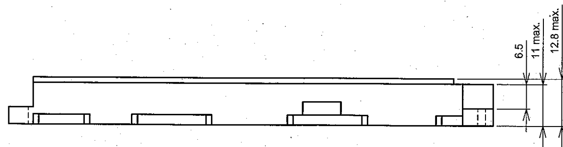
Front View
