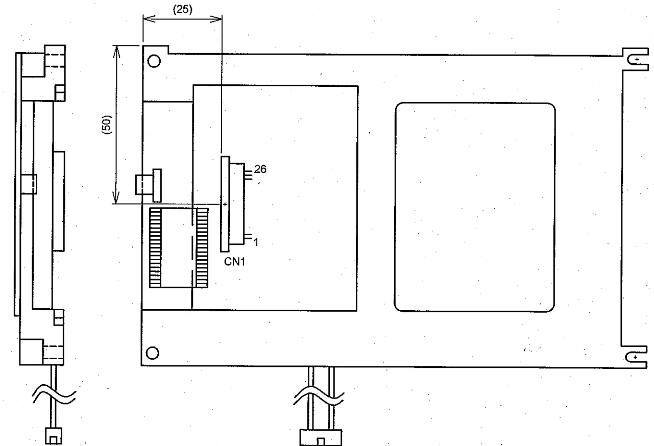
Rear View
