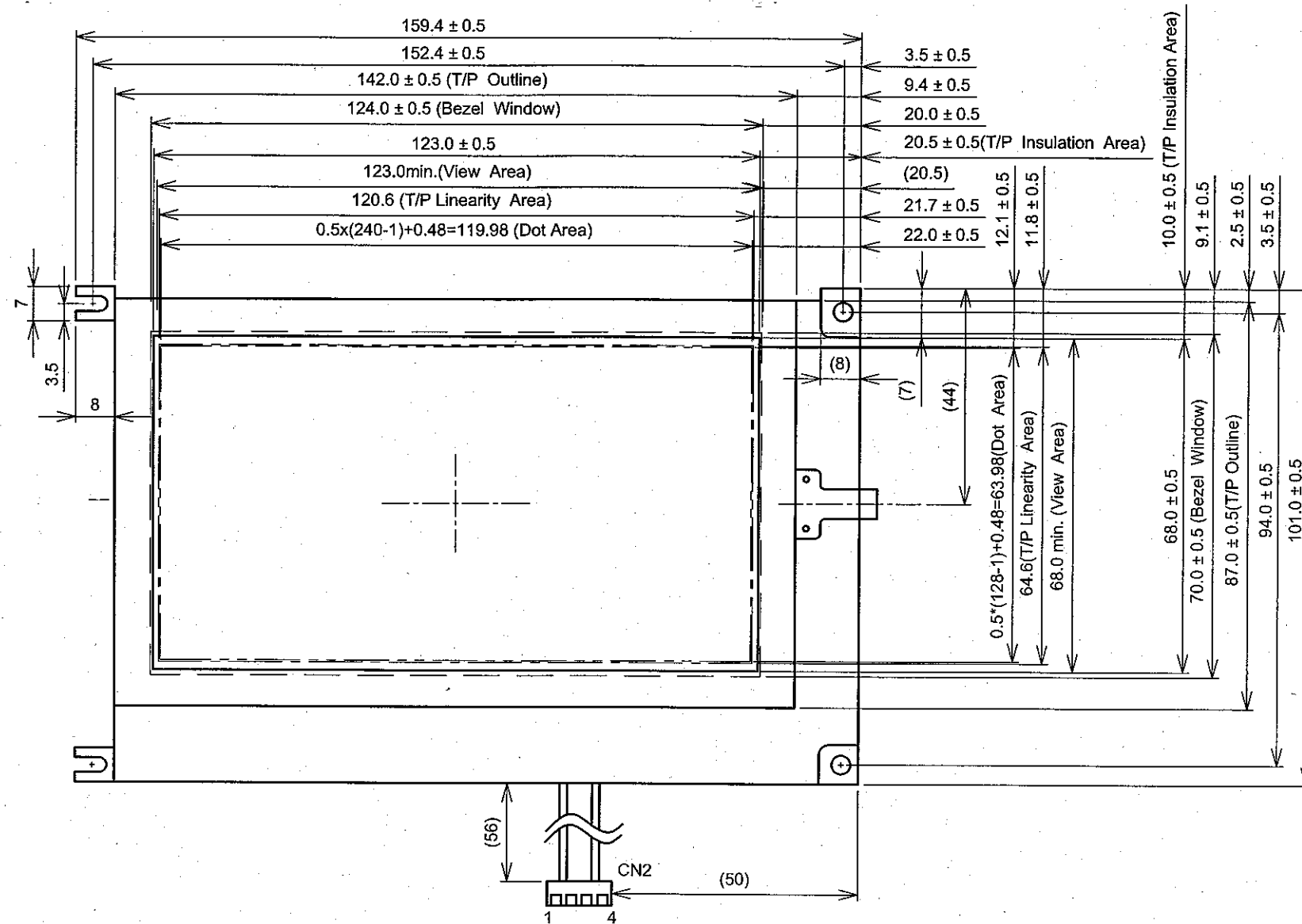
Front View
