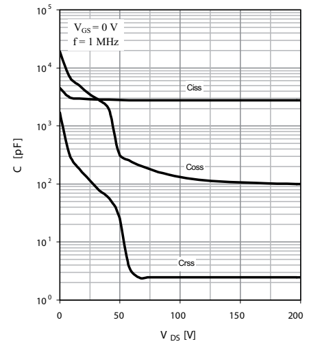
Fig. 9 Typ. capacitances
