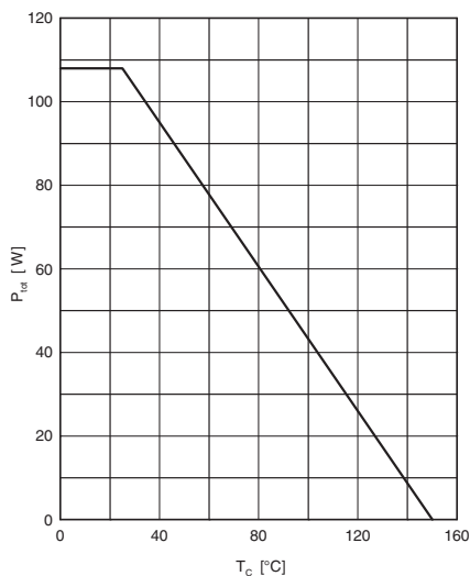
Fig. 1 Power dissipation
