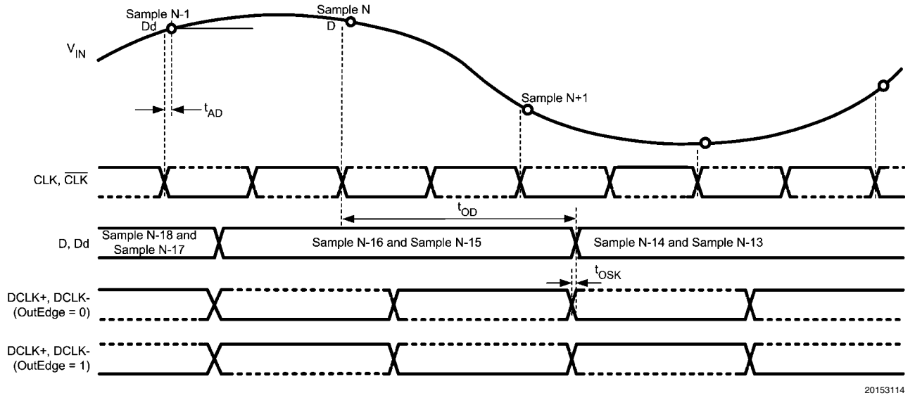
FIGURE 3. ADC081500 Timing — SDR Clocking
