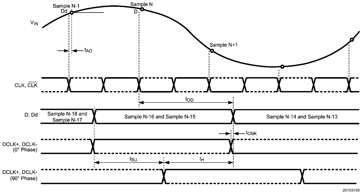
FIGURE 4. ADC081500 Timing — DDR Clocking
