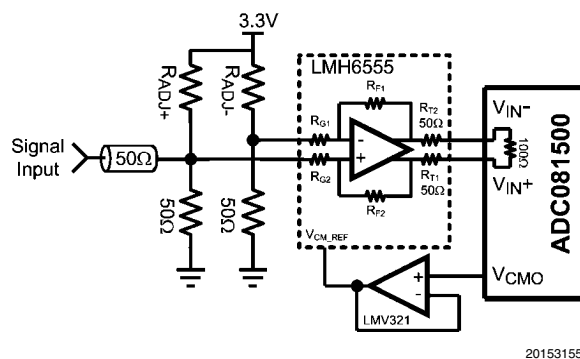
FIGURE 13. Example of Servoing the Analog Input with V_{CM0}
