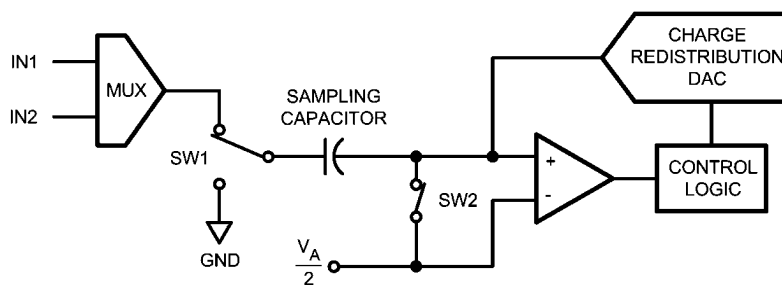
FIGURE 1. ADC102S021 in Track Mode
