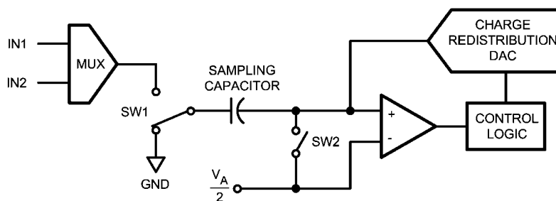
FIGURE 2. ADC102S021 in Hold Mode
