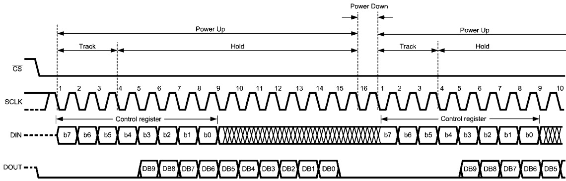
ADC102S051 Operational Timing Diagram
