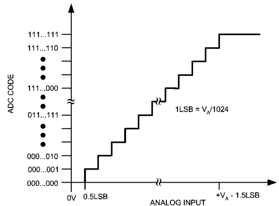
FIGURE 3. Ideal Transfer Characteristic performance. To keep noise off the supply, use a dedicated linear regulator for this device, or provide sufficient decoupling from other circuitry to keep noise off the ADC104S051 supply pin. Because of the ADC104S051's low power requirements, it is also possible to use a precision reference as a power supply to maximize performance. The four-wire interface is also shown connected to a microprocessor or DSP.
