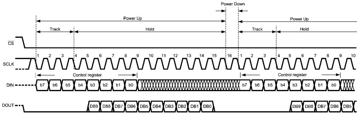
ADC104S051 Operational Timing Diagram
