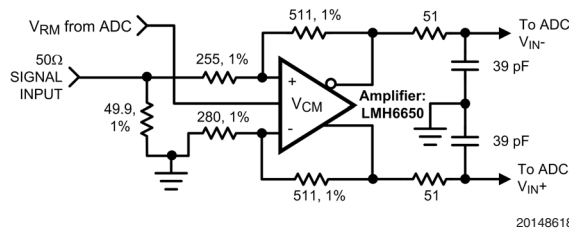
FIGURE 6. Optional Amplifier Differential Drive Circuit
