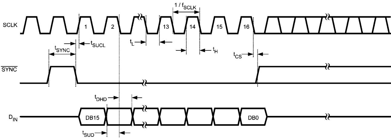
FIGURE 2. DAC121S101 Timing
