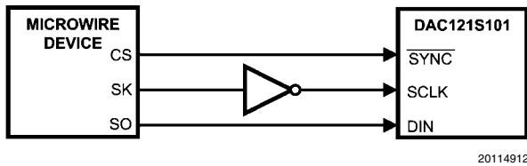
FIGURE 8. Microwire Interface
