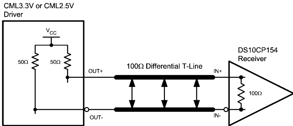
Typical CML Driver DC-Coupled Interface to DS10CP154 Input
