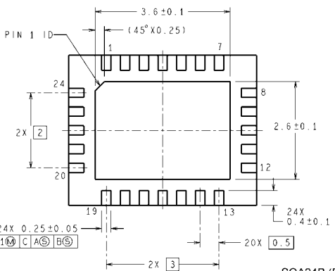
24 Lead LLP NS Package Number SQA24B
