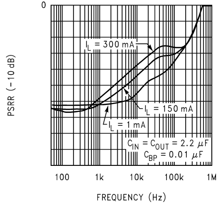
Ripple Rejection ( V_{IN} = V_{OUT} + 1\text{V} )
