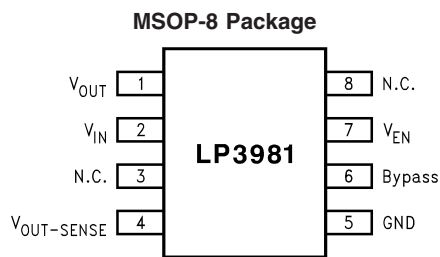
Top View See NS Package Number MUA008AE
