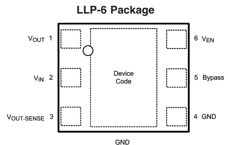
Top View See NS Package Number LDC06D
