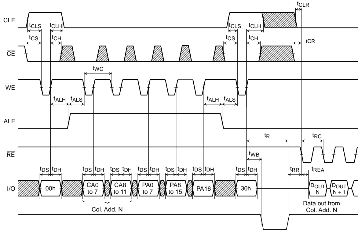
Read Cycle Timing Diagram
