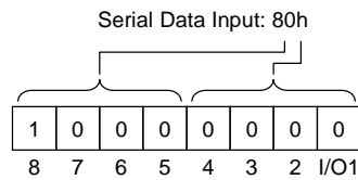
HEX data bit assignment (Example)
