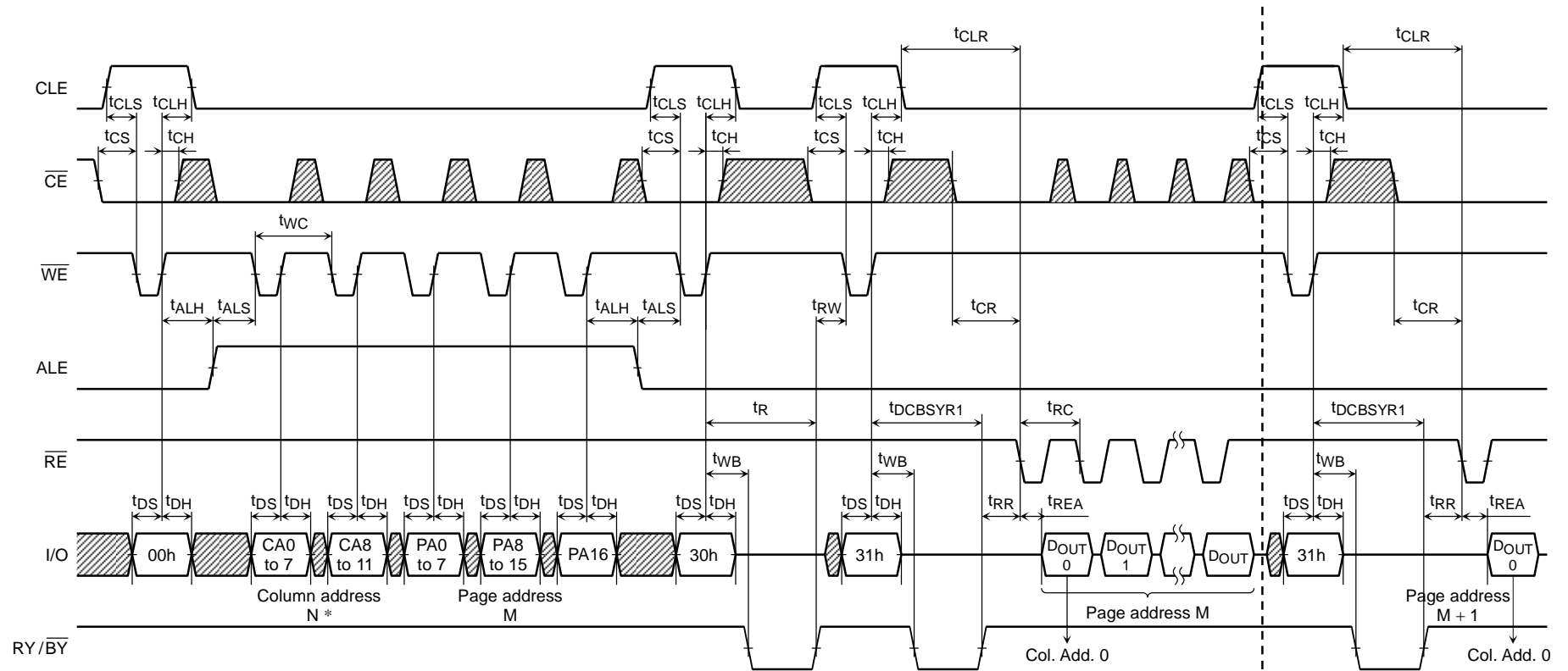
Read Cycle with Data Cache Timing Diagram (1/2)
