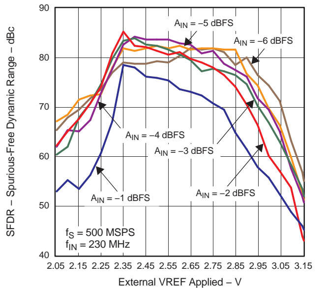
Figure 54. ADS5463 SFDR versus External VREF and AIN
