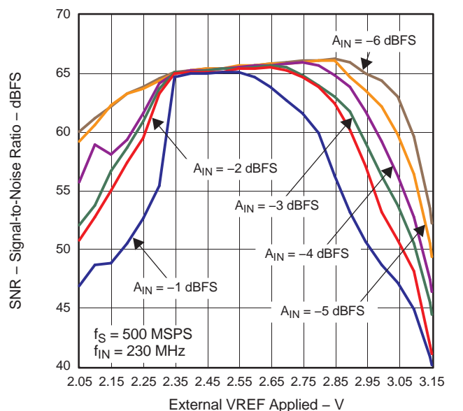
Figure 55. ADS5463 SNR versus External VREF and AIN
