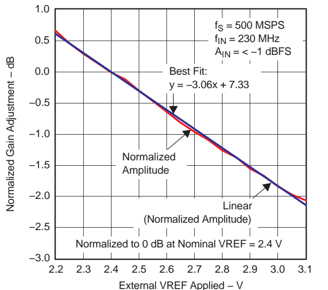
Figure 53. ADS5463 Signal Gain Adjustment versus External Reference (VREF)
