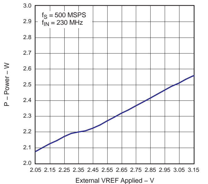
Figure 56. Total Power Consumption versus External VREF
