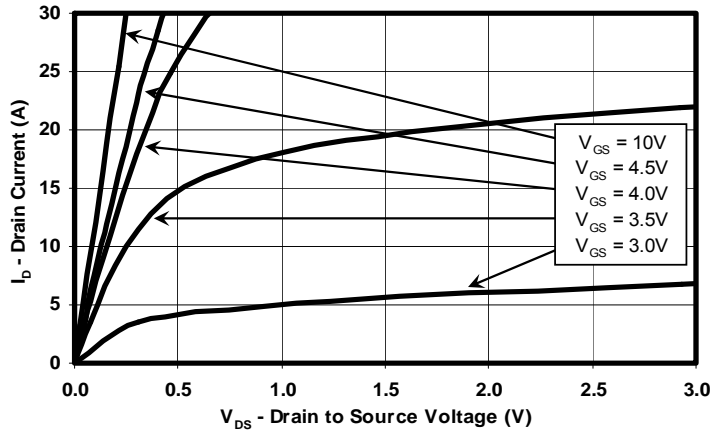
Figure 2: Saturation Characteristics
