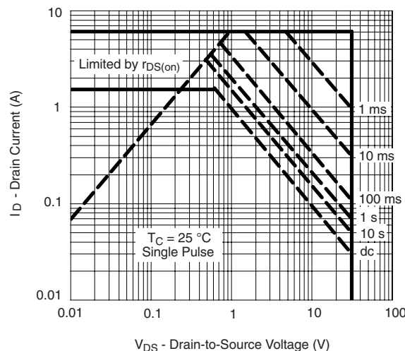
Safe Operating Area, Junction-to-Ambient *V_{GS} > \text{minimum } V_{GS} \text{ at which } r_{DS(on)} \text{ is specified}
