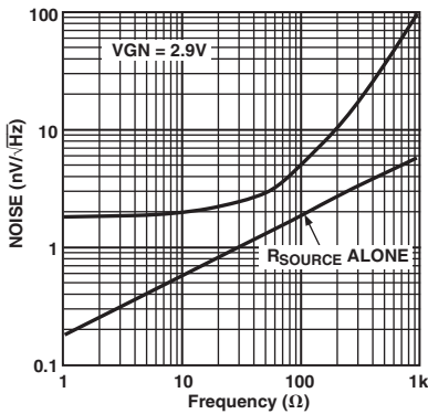
TPC 16. Input Referred Noise vs. R_{SOURCE}
