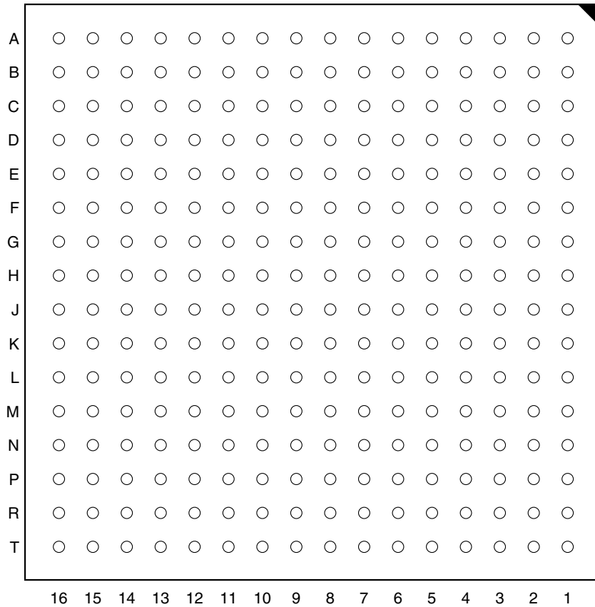
256-ball 1.0 mm Pitch – Bottom View
