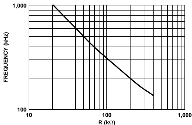
FIGURE 6. FREQUENCY vs FS RESISTOR
