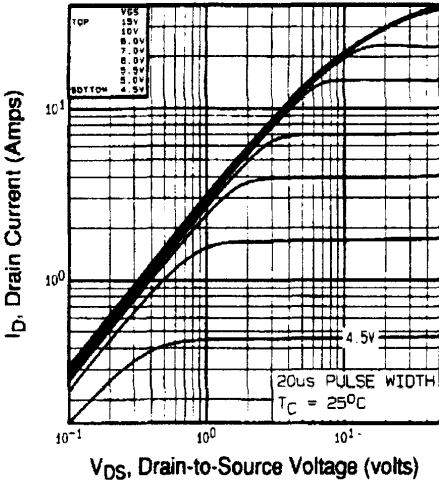
Fig 1. Typical Output Characteristics, T_C=25^\circ C
