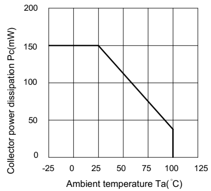
Fig. 8 Collector Power Dissipation vs. Ambient Temperature
