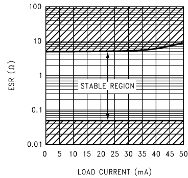
FIGURE 3. ESR Curve for C_{OUT} = 2.2\mu F
