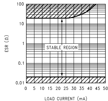
FIGURE 5. ESR Curve for C_{OUT} = 10\mu F
