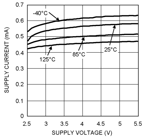
I_S vs. V_S Over Temperature
