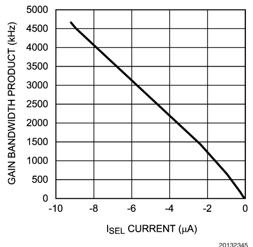
Gain Bandwidth Product vs. I_{SEL}
