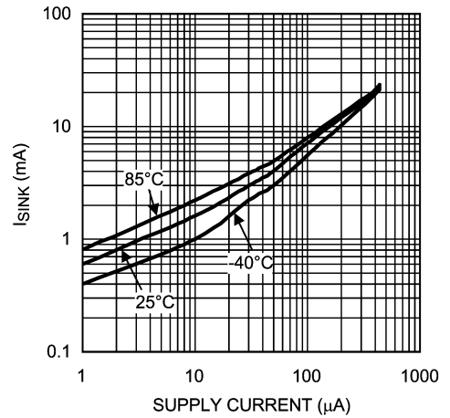
I_{SINK} vs. Supply Current
