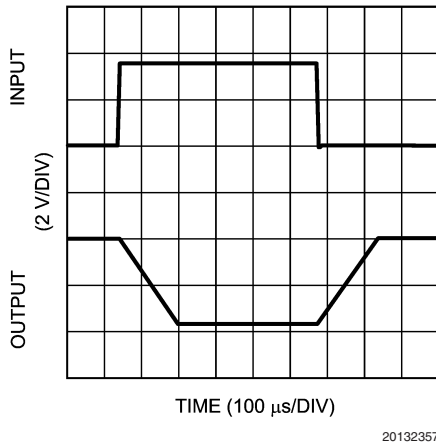
Large Signal Inverting Response (Low Power Mode)
