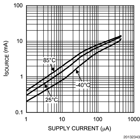
I_{SOURCE} vs. Supply Current
