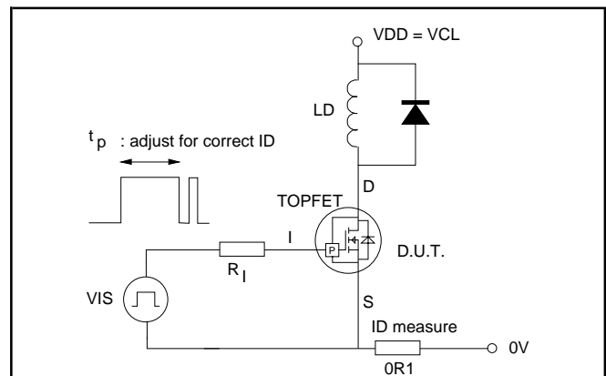
Fig.23. Test circuit for inductive load switching times.
