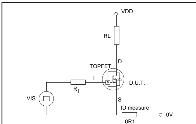
Fig.20. Test circuit for resistive load switching times.
