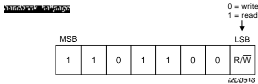
Fig.7 Address byte.
