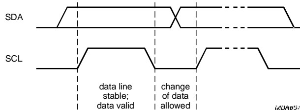
Fig.9 Bit transfer.
