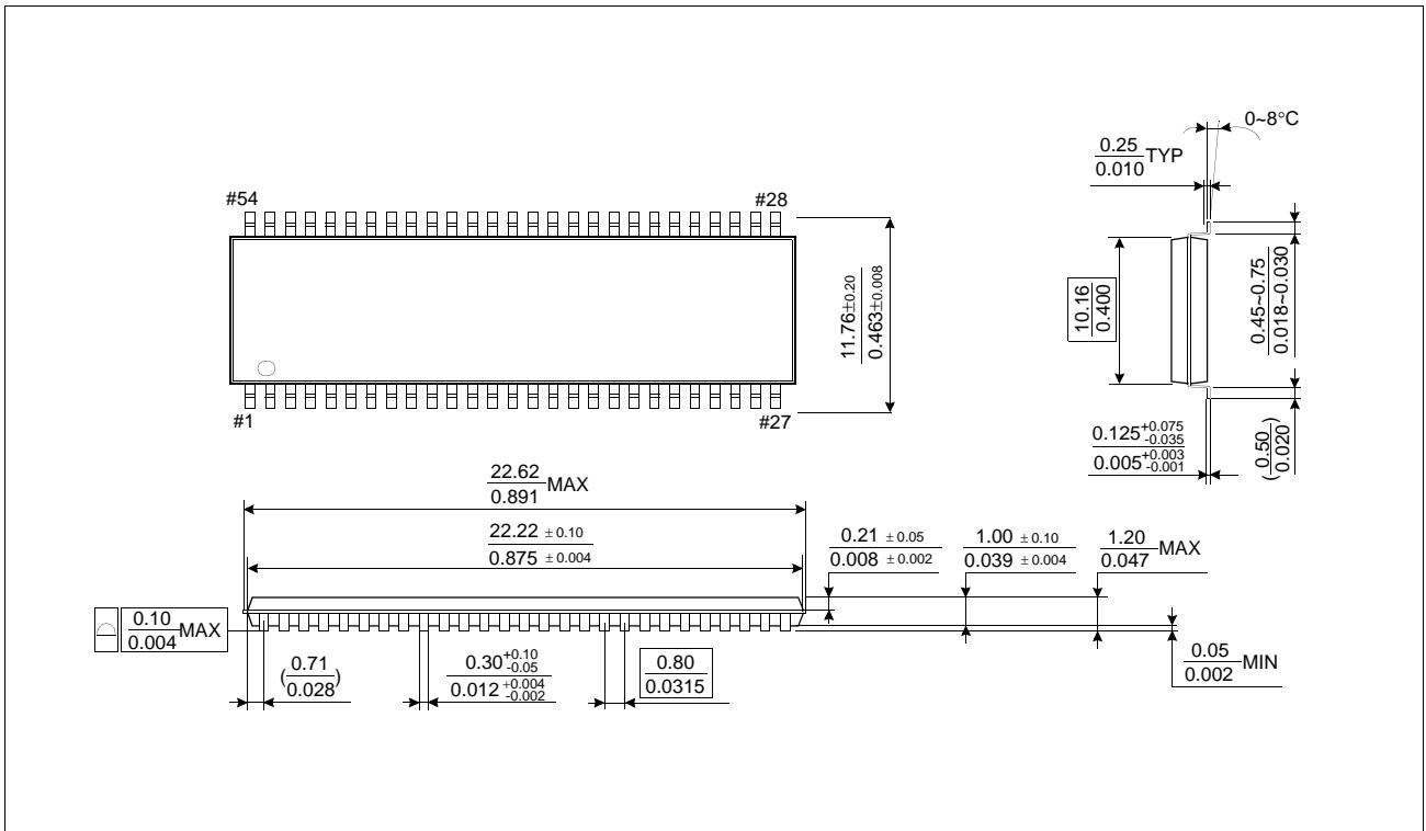
54Pin TSOP Package Dimension
