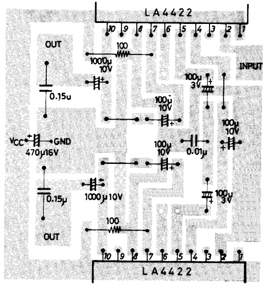
Sample Printed Circuit Pattern (45 x 43mm 3 , Cu-foiled side)
