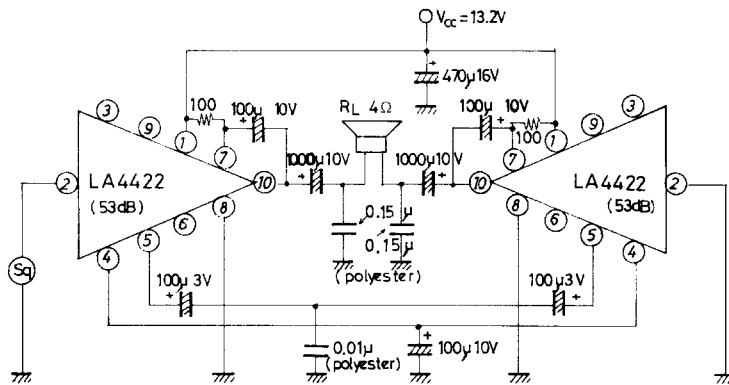
Sample Application Circuit 2. 18W typ. (V CC =13.2V, R L =4Ω) BTL amplifier
