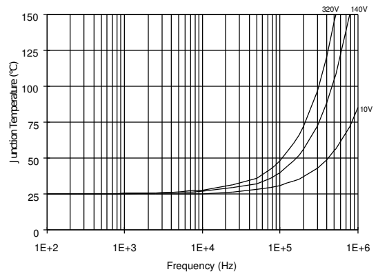
Figure 33. IR2113 T J vs. Frequency (IRFBC30) R GATE = 22Ω, V CC = 15V
