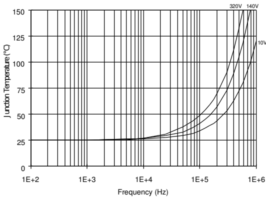
Figure 34. IR2113 T J vs. Frequency (IRFBC40) R GATE = 15Ω, V CC = 15V
