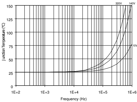
Figure 32. IR2113 T J vs. Frequency (IRFBC20) R GATE = 33Ω, V CC = 15V
