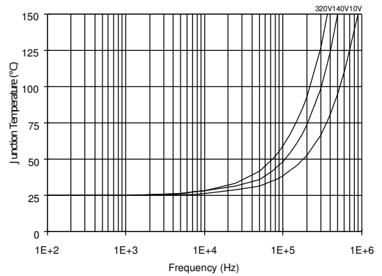
Figure 35. IR2113 T J vs. Frequency (IRFBE50) R GATE = 10Ω, V CC = 15V
