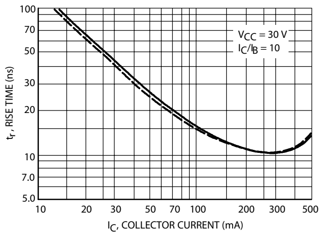
FIG 6. Rise Time
