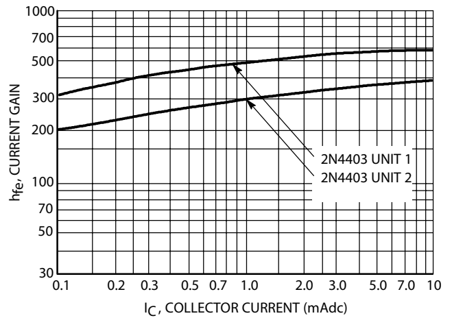
FIG. 10 Current Gain
