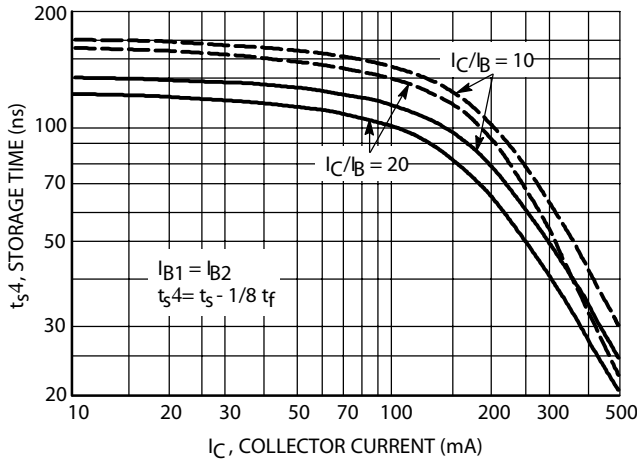
FIG. 7 Storage Time
