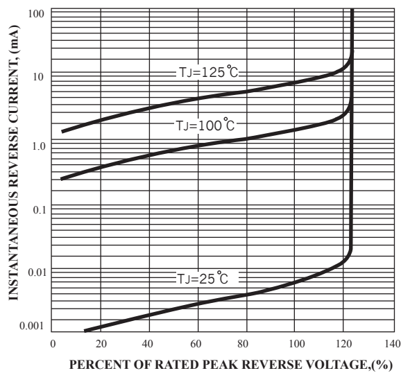
FIG.5-TYPICAL REVERSE CHARACTERISTICS
