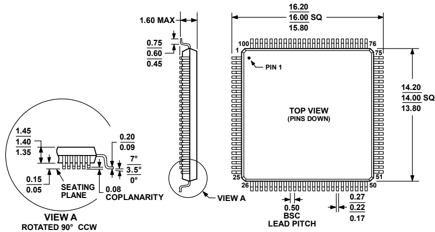
Figure 35. 100-Lead Low Profile Quad Flat Package [LQFP] (ST-100) Dimensions shown in millimeters
