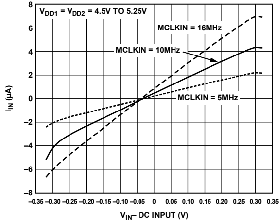
Figure 18. I_{IN} vs. V_{IN}
