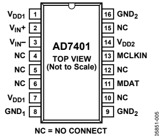
Figure 5. 16-Lead SOIC_W Pin Configuration
