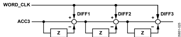
Figure 27. Differentiator
