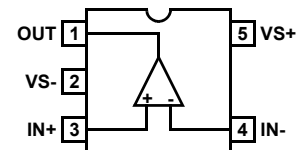
EL5161 (5-PIN SOT-23, SC-70) TOP VIEW
