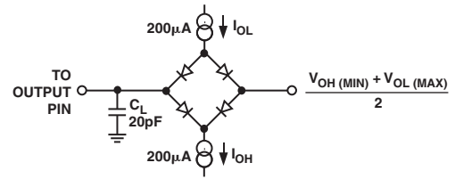
Figure 3. Load Circuit for SDO Timing Specifications
