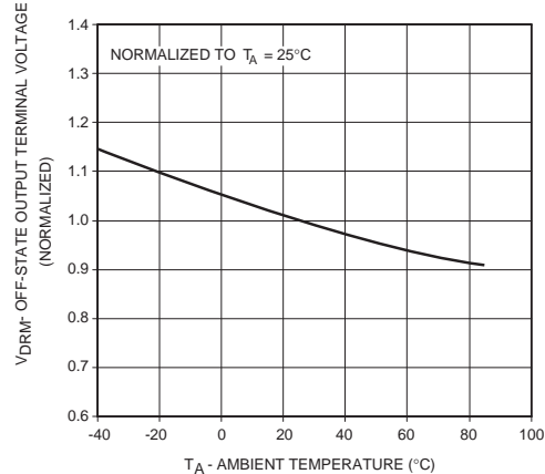
Fig. 6 Off-state Output Terminal Voltage vs. Ambient Temperature
