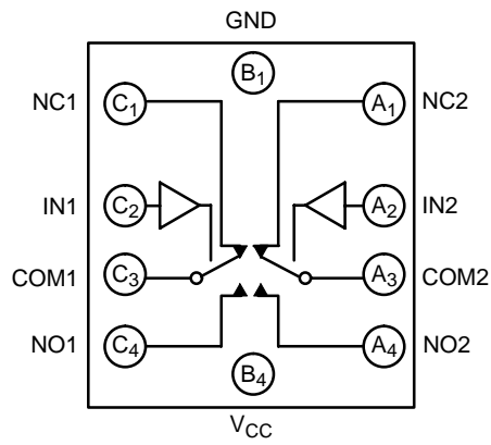
Figure 2. Pin Connections and Logic Diagram (Microbump-10)
