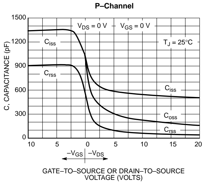
Figure 7. Capacitance Variation
