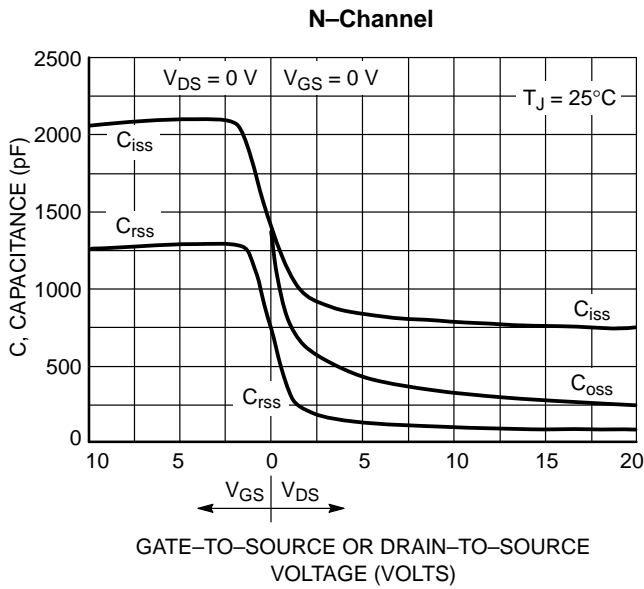
Figure 7. Capacitance Variation
