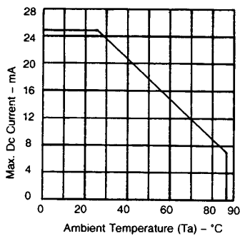
Fig. 4. Maximum Forward Allowable DC Current Per Segment vs. of Ambient Temperature
