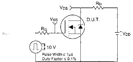
Fig 10a. Switching Time Test Circuit
