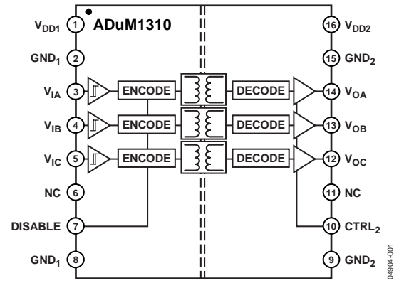
Figure 1. ADuM1310
